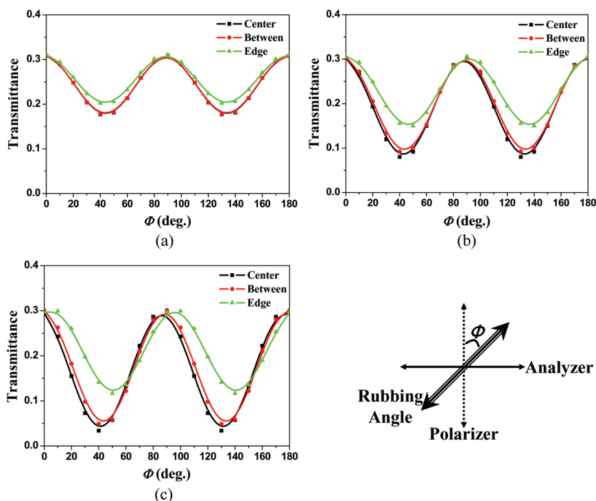
FIGURE 4 Light modulation according to the electrode structures; (a) w = 1 \mu\text{m} , l = 1.5 \mu\text{m} , (b) w = 2 \mu\text{m} , l = 3 \mu\text{m} , and (c) w = 3 \mu\text{m} , l = 4.5 \mu\text{m} .
